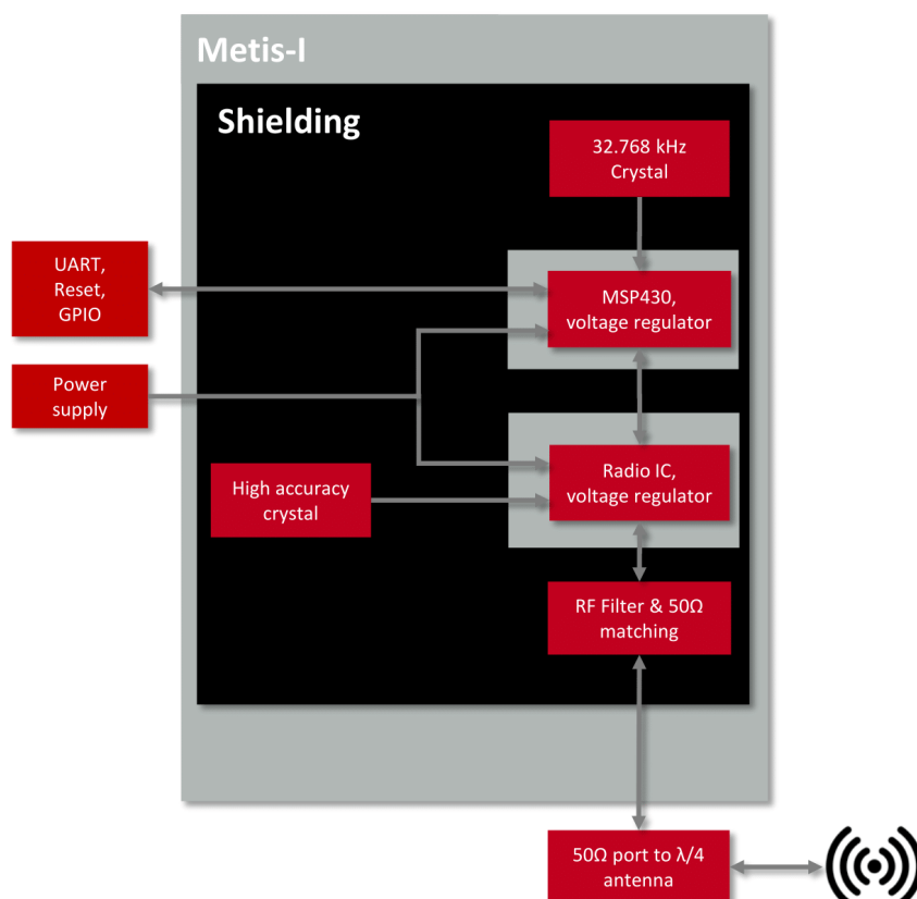
Figure 1: Block diagram of the Metis-I module
